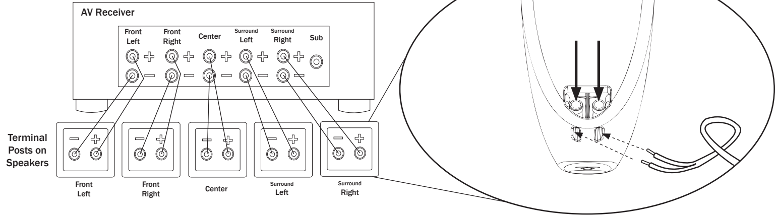
FIGURE 3 – SPEAKER WIRE HOOKUP
