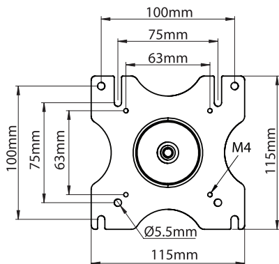
INTERFACE PLATE
