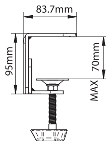
DESK CLAMP
